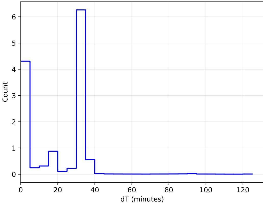
too_elab_r32_d2_gz_v3.4_10yrs All sky: DeltaT Histogram 1e6
