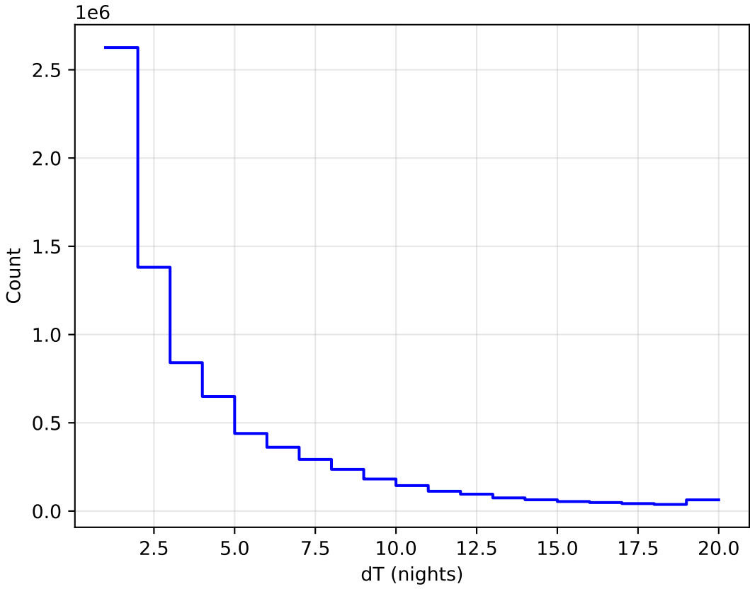
too_elab_r32_d2_gz_v3.4_10yrs WFD all bands: DeltaNight Histogram
