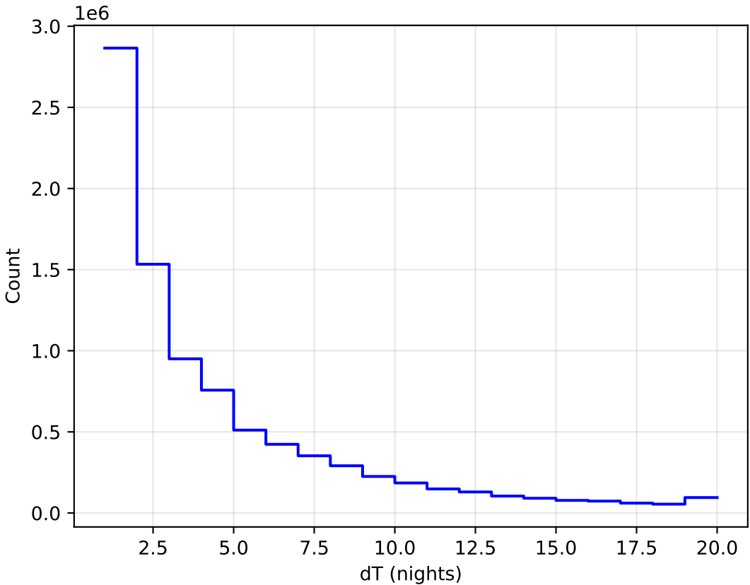
too_elab_r32_d2_gz_v3.4_10yrs All sky all bands: DeltaNight Histogram
