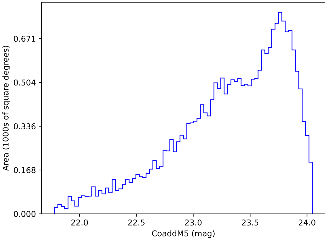
too_elab_r32_d2_gz_v3.4_10yrs Yr 3-4 y band: CoaddM5
