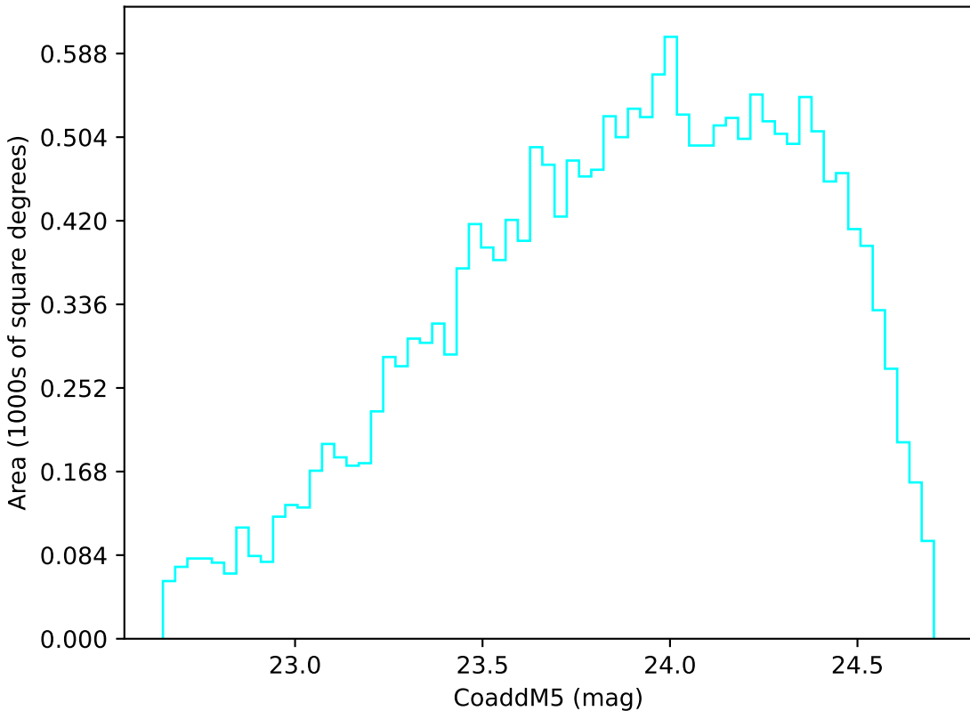
too_elab_r32_d2_gz_v3.4_10yrs Yr 3-4 u band: CoaddM5
