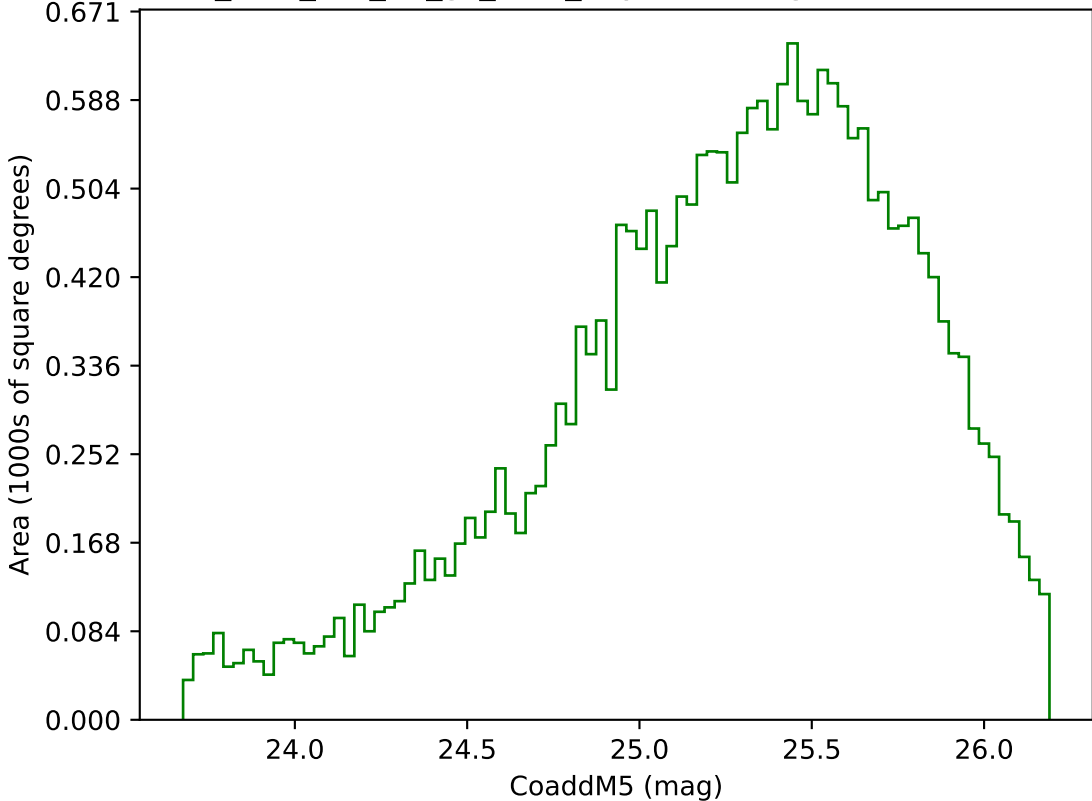
too_elab_r32_d2_gz_v3.4_10yrs Yr 3-4 g band: CoaddM5
