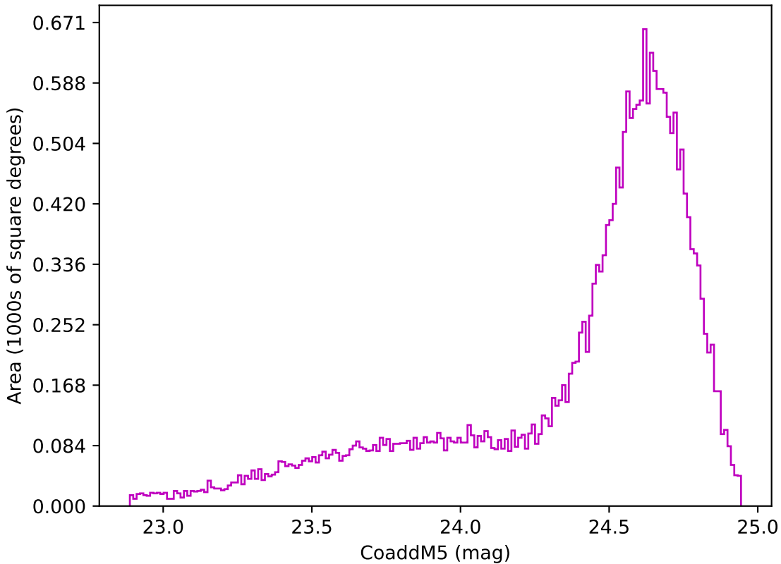
too_elab_r32_d2_gz_v3.4_10yrs Yr 1 z band: CoaddM5
