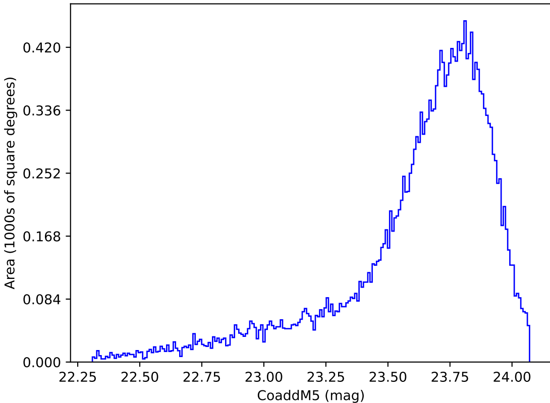
too_elab_r32_d2_gz_v3.4_10yrs Yr 1 y band: CoaddM5
