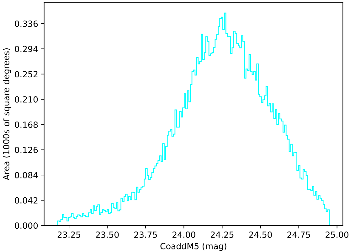
too_elab_r32_d2_gz_v3.4_10yrs Yr 1 u band: CoaddM5
