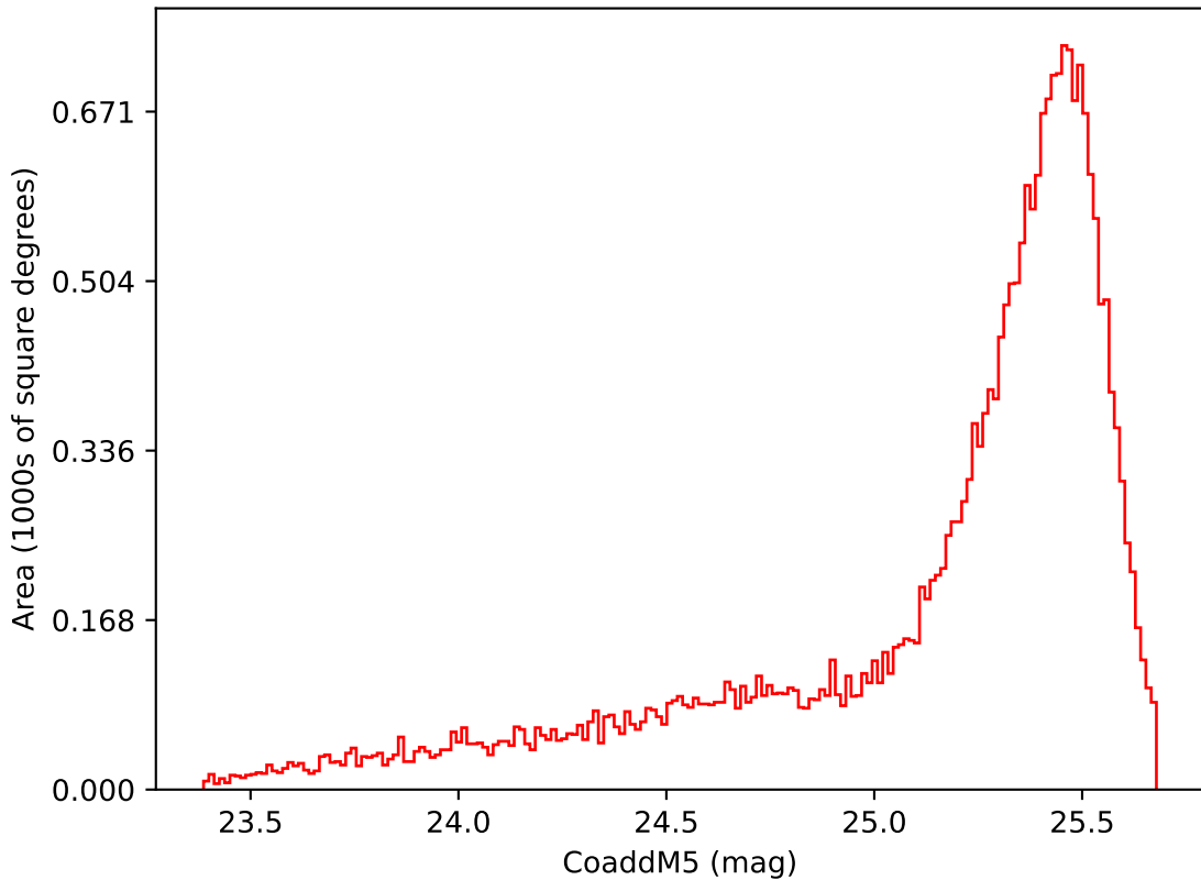
too_elab_r32_d2_gz_v3.4_10yrs Yr 1 i band: CoaddM5
