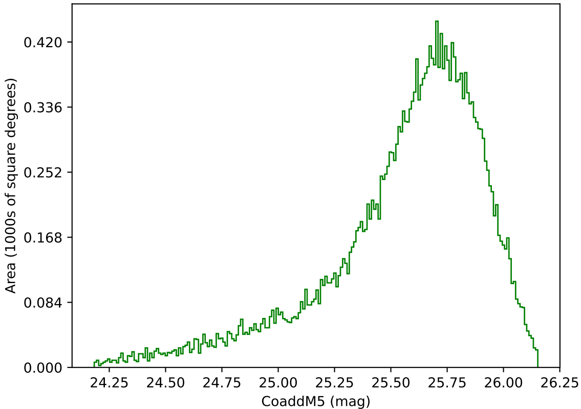
too_elab_r32_d2_gz_v3.4_10yrs Yr 1 g band: CoaddM5
