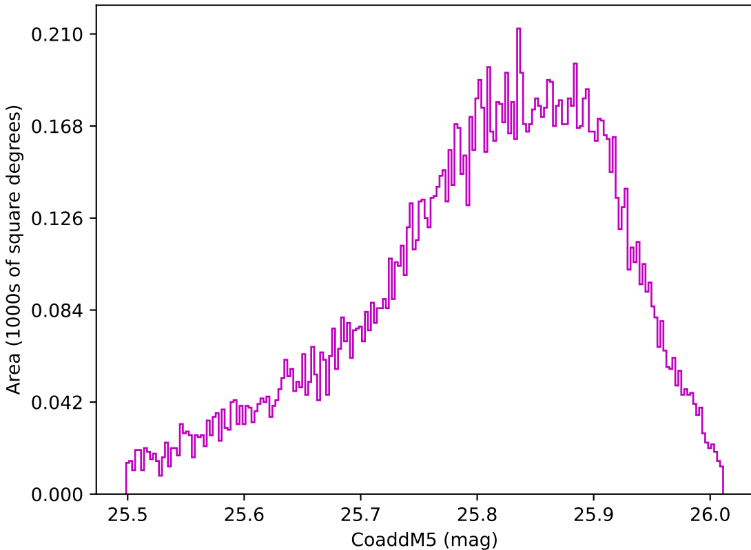
too_elab_r32_d2_gz_v3.4_10yrs WFD z band: CoaddM5
