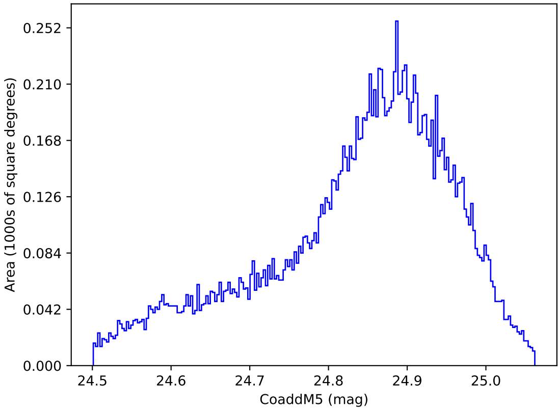
too_elab_r32_d2_gz_v3.4_10yrs WFD y band: CoaddM5
