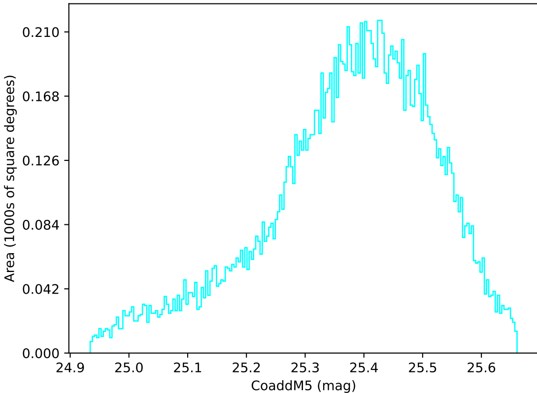
too_elab_r32_d2_gz_v3.4_10yrs WFD u band: CoaddM5
