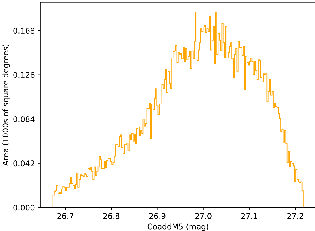
too_elab_r32_d2_gz_v3.4_10yrs WFD r band: CoaddM5
