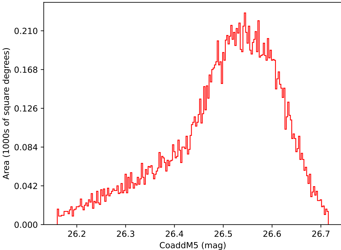
too_elab_r32_d2_gz_v3.4_10yrs WFD i band: CoaddM5
