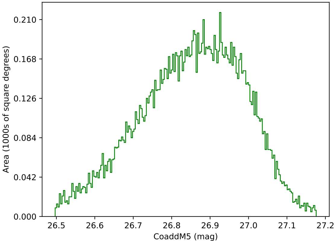
too_elab_r32_d2_gz_v3.4_10yrs WFD g band: CoaddM5
