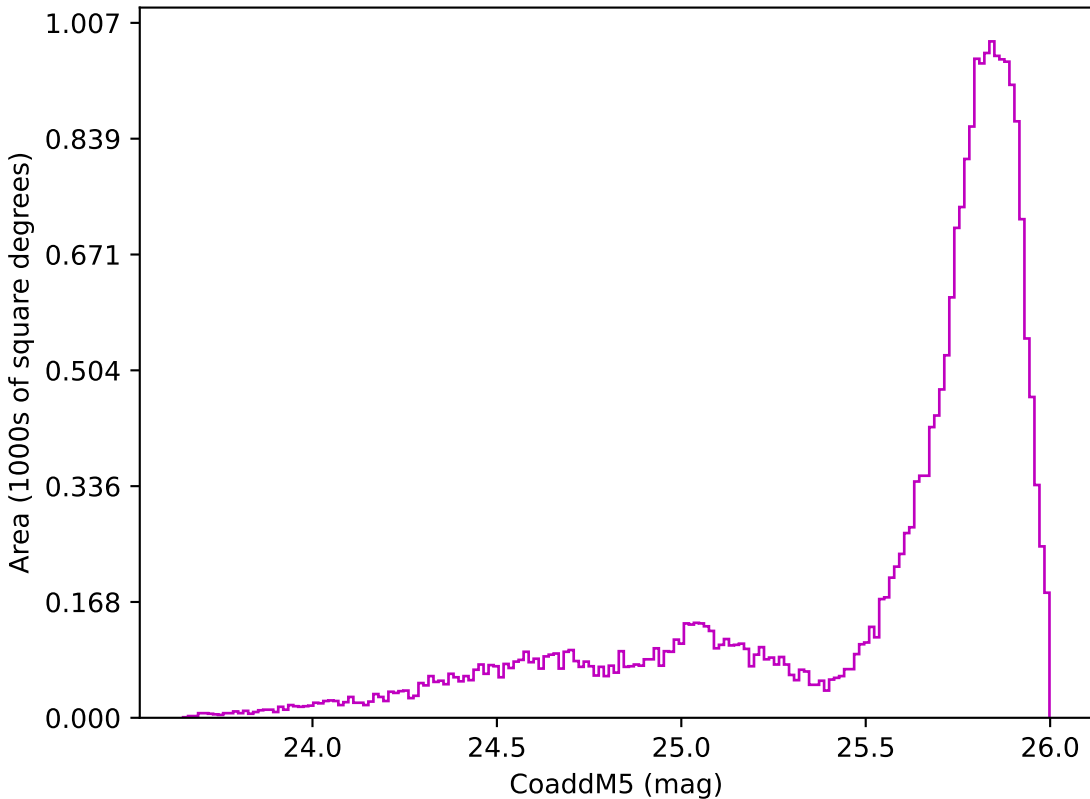
too_elab_r32_d2_gz_v3.4_10yrs All sky z band: CoaddM5
