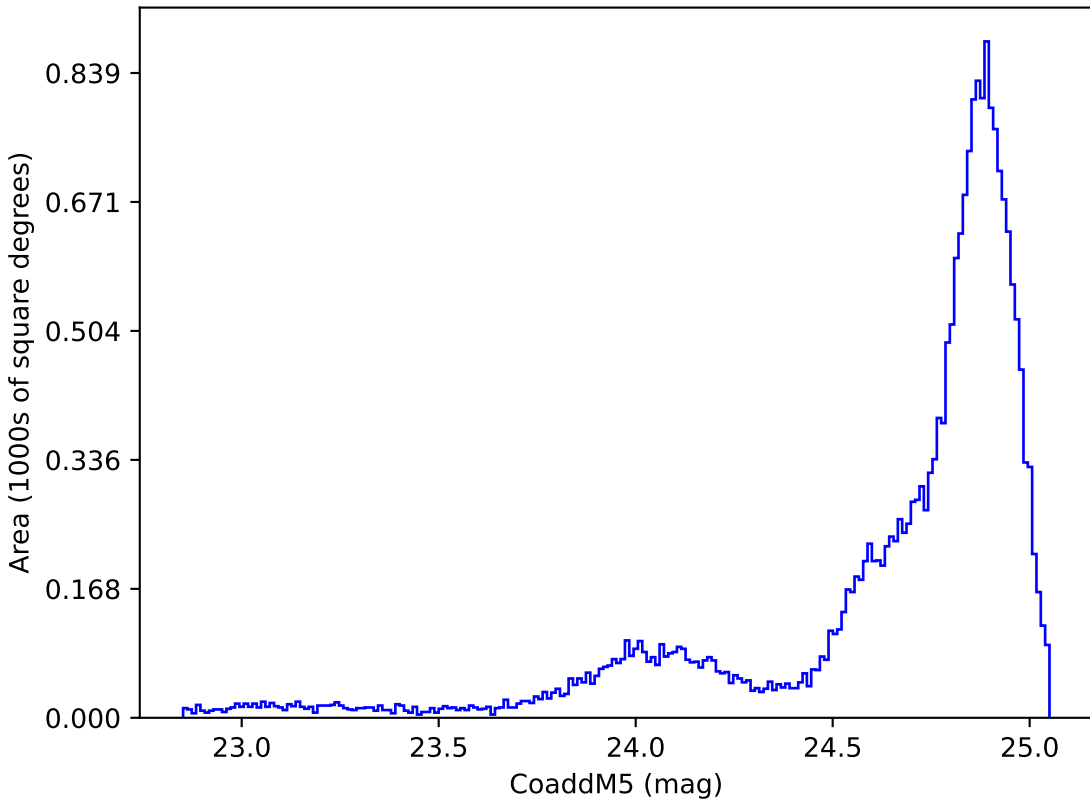
too_elab_r32_d2_gz_v3.4_10yrs All sky y band: CoaddM5
