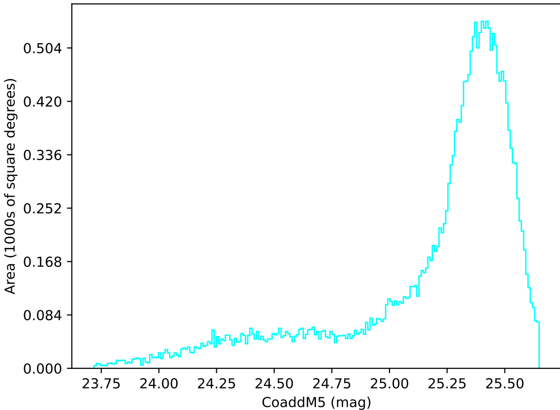
too_elab_r32_d2_gz_v3.4_10yrs All sky u band: CoaddM5
