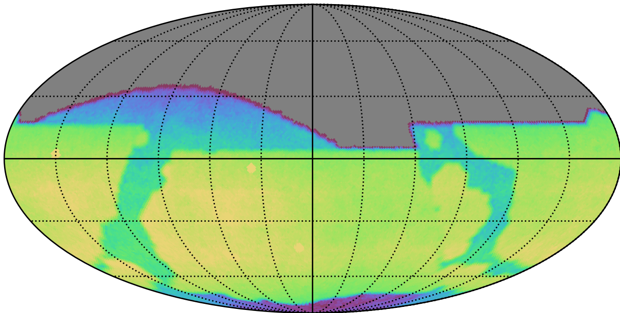
too_elab_r32_d2_gz_v3.4_10yrs All sky r band: CoaddM5
