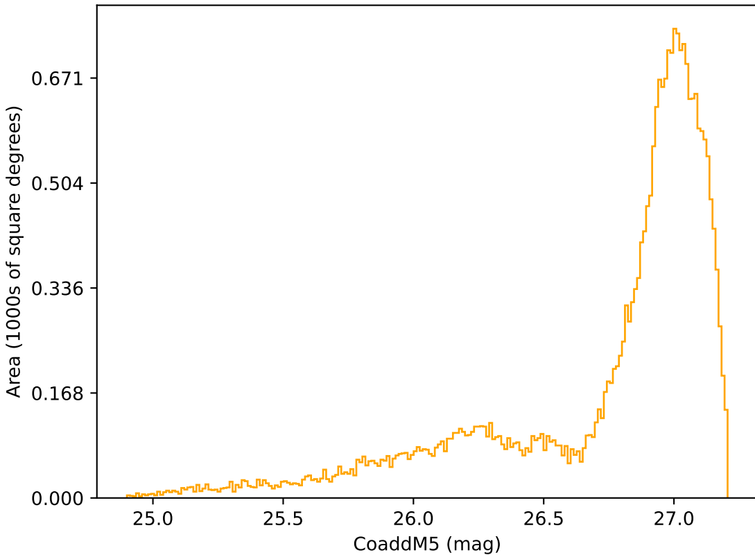
too_elab_r32_d2_gz_v3.4_10yrs All sky r band: CoaddM5
