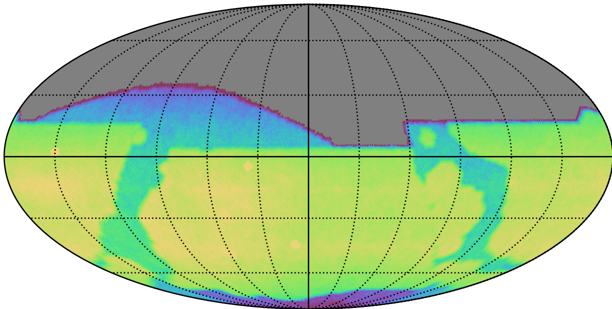
too_elab_r32_d2_gz_v3.4_10yrs All sky i band: CoaddM5
