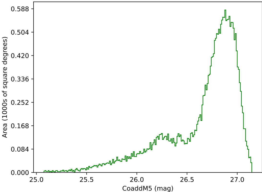
too_elab_r32_d2_gz_v3.4_10yrs All sky g band: CoaddM5
