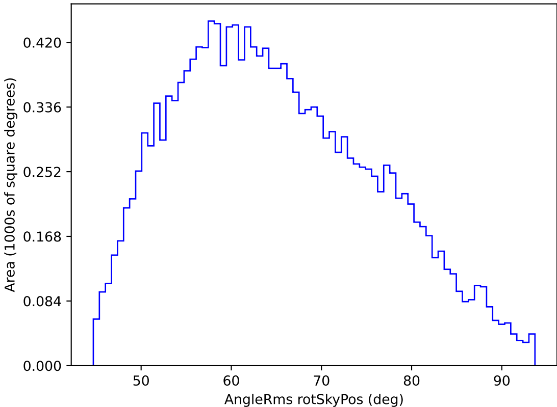
too_elab_r32_d2_gz_v3.4_10yrs WFD u band: AngleRms rotSkyPos
