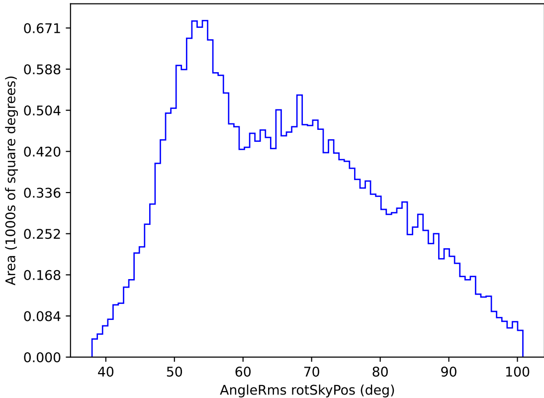
too_elab_r32_d2_gz_v3.4_10yrs All sky g band: AngleRms rotSkyPos
