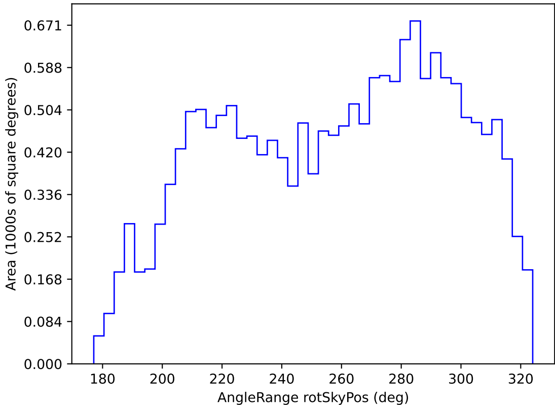
too_elab_r32_d2_gz_v3.4_10yrs WFD u band: AngleRange rotSkyPos
