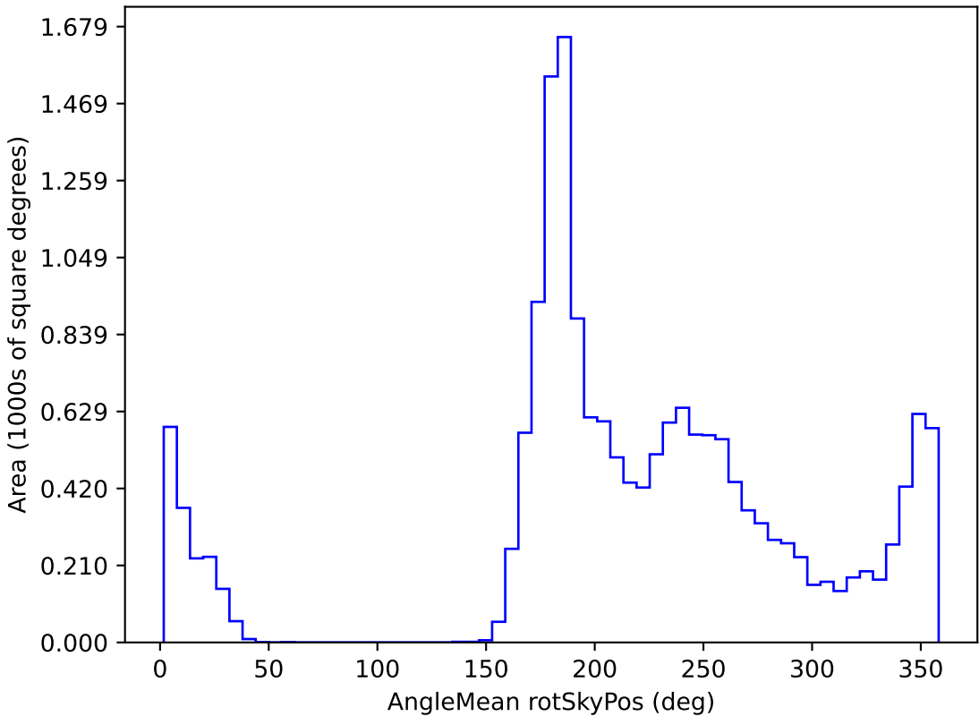
too_elab_r32_d2_gz_v3.4_10yrs WFD z band: AngleMean rotSkyPos
