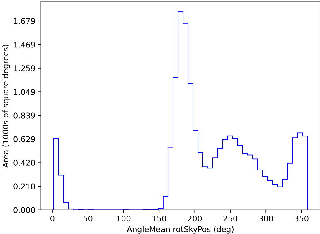
too_elab_r32_d2_gz_v3.4_10yrs WFD y band: AngleMean rotSkyPos
