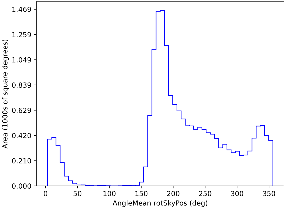
too_elab_r32_d2_gz_v3.4_10yrs WFD u band: AngleMean rotSkyPos
