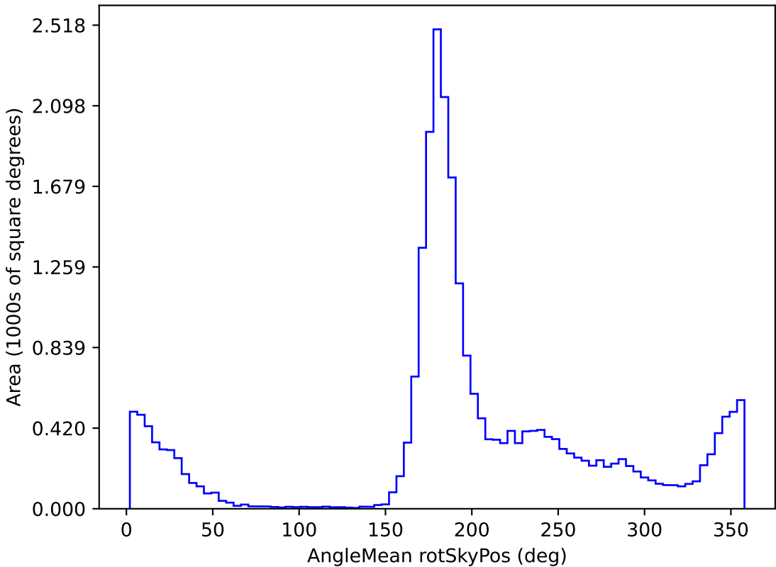
too_elab_r32_d2_gz_v3.4_10yrs All sky r band: AngleMean rotSkyPos
