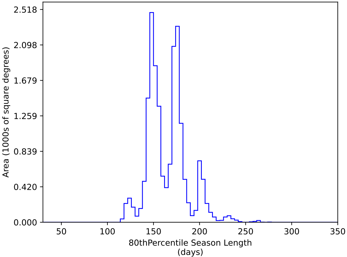
too_elab_r32_d2_gz_v3.4_10yrs WFD y band: 80thPercentile Season Length
