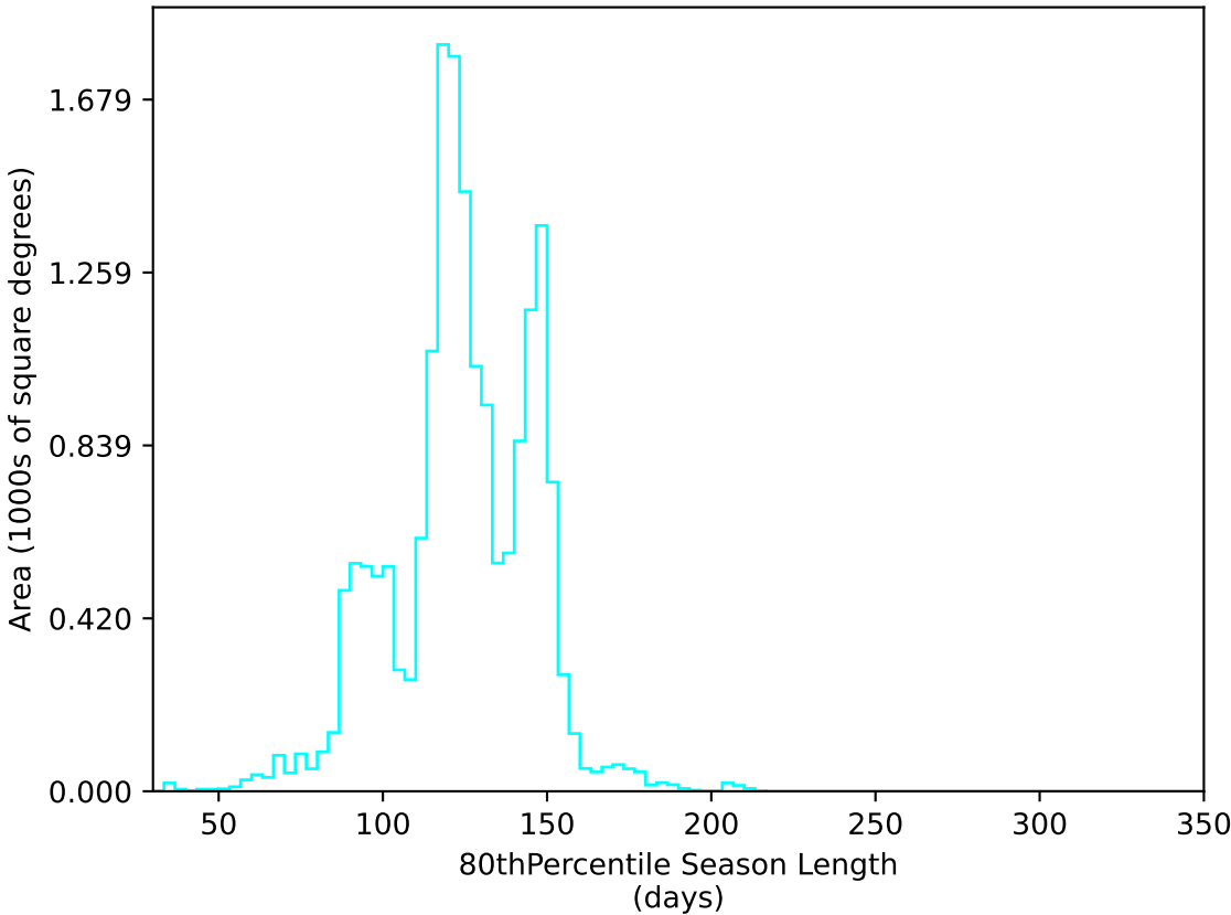
too_elab_r32_d2_gz_v3.4_10yrs WFD u band: 80thPercentile Season Length
