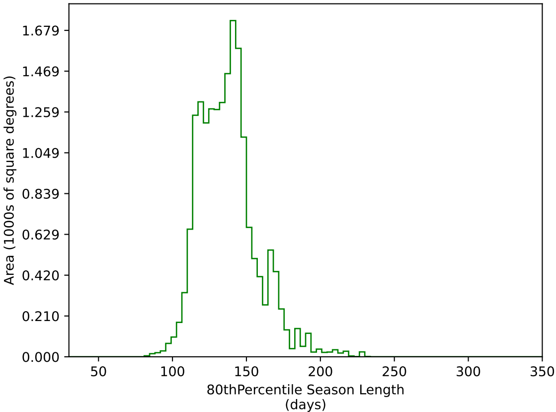
too_elab_r32_d2_gz_v3.4_10yrs WFD g band: 80thPercentile Season Length
