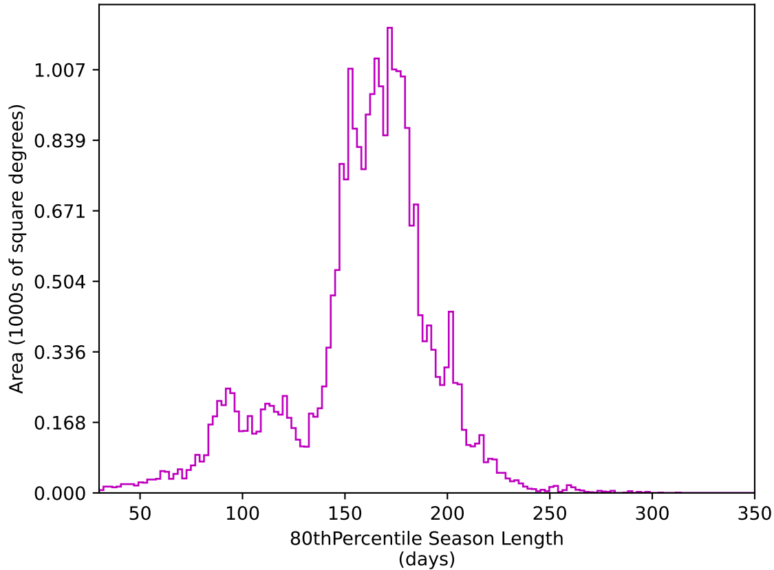
too_elab_r32_d2_gz_v3.4_10yrs All sky z band: 80thPercentile Season Length
