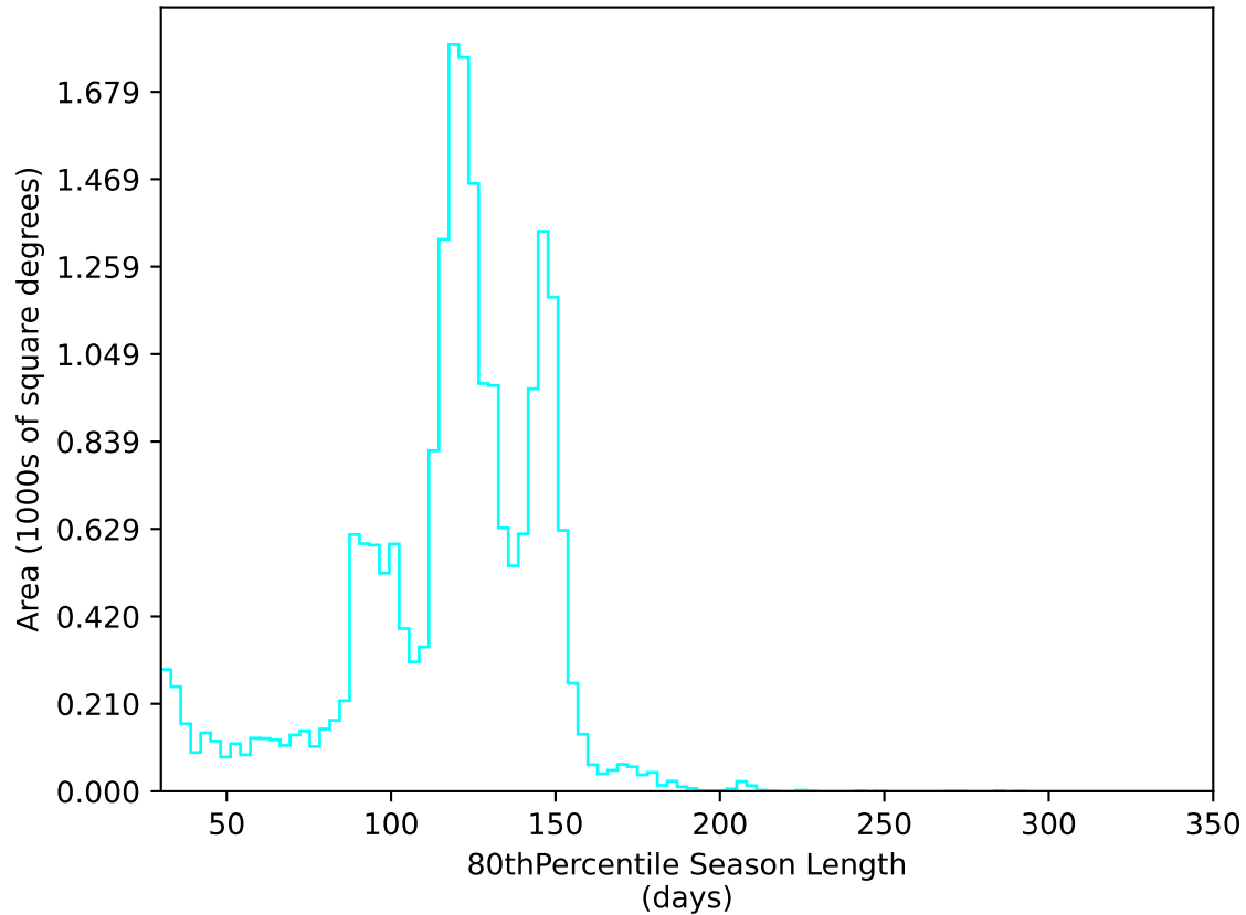
too_elab_r32_d2_gz_v3.4_10yrs All sky u band: 80thPercentile Season Length
