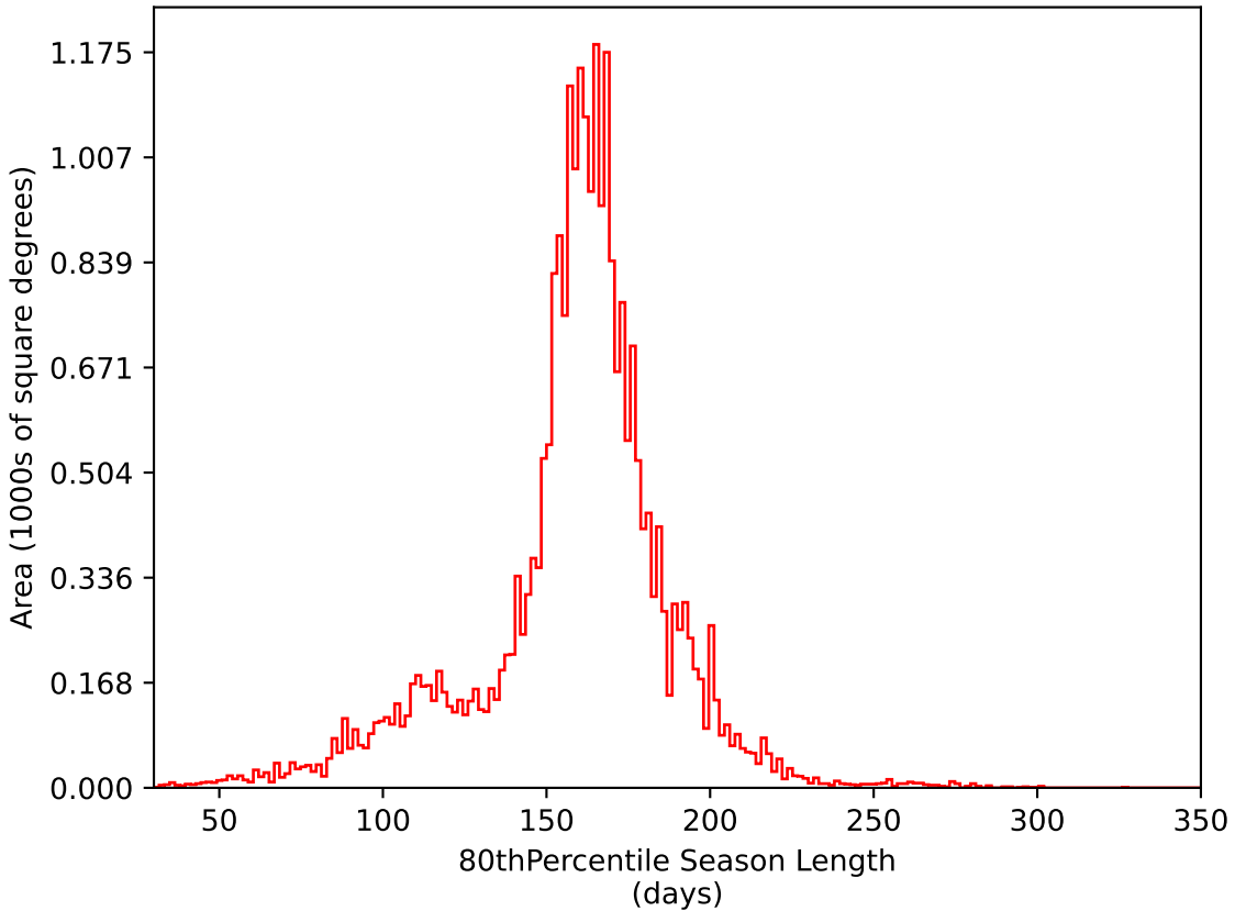
too_elab_r32_d2_gz_v3.4_10yrs All sky i band: 80thPercentile Season Length
