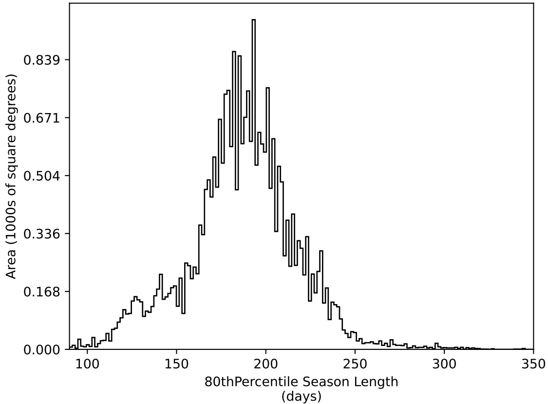
too_elab_r32_d2_gz_v3.4_10yrs All sky all bands: 80thPercentile Season Length
