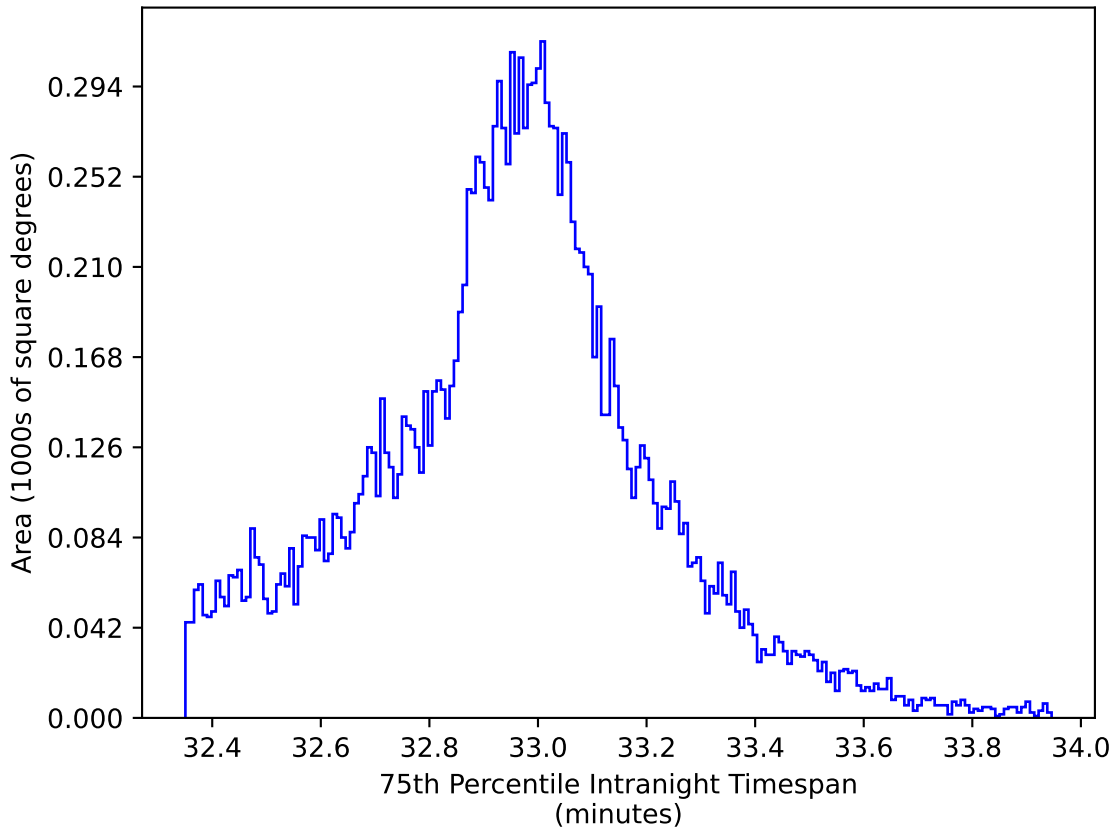
too_elab_r32_d2_gz_v3.4_10yrs WFD y band: 75th Percentile Intranight Timespan
