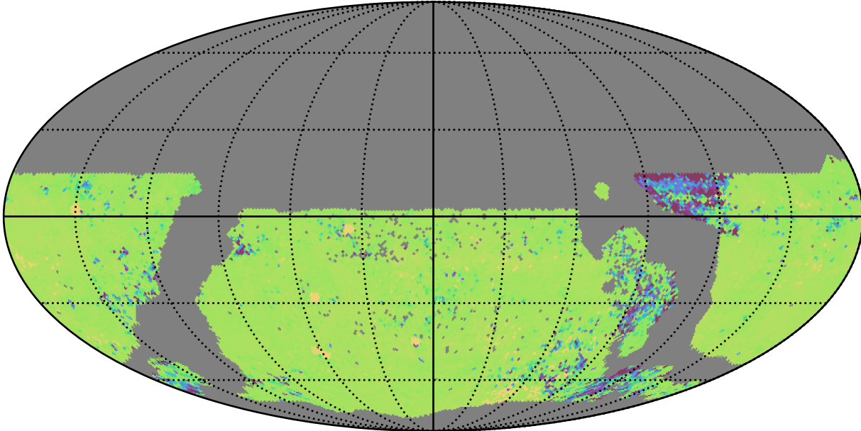
too_elab_r32_d2_gz_v3.4_10yrs WFD ug bands: 75th Percentile Intranight Timespan
