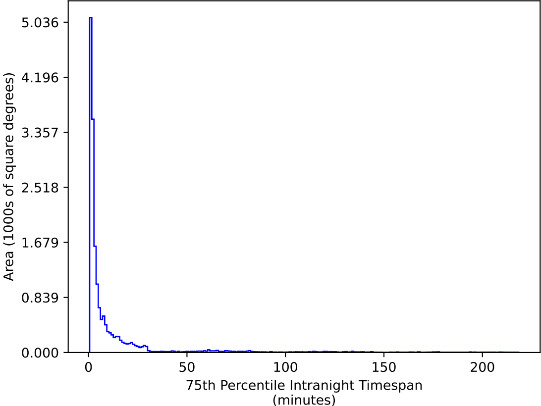
too_elab_r32_d2_gz_v3.4_10yrs WFD u band: 75th Percentile Intranight Timespan
