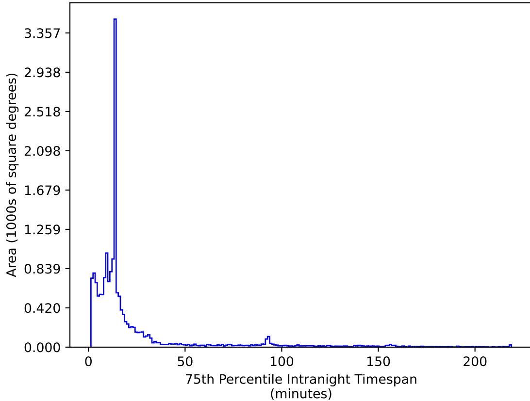
too_elab_r32_d2_gz_v3.4_10yrs WFD i band: 75th Percentile Intranight Timespan
