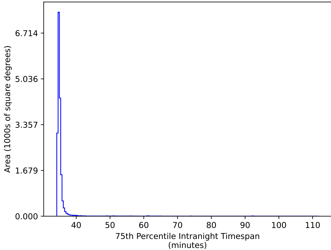
too_elab_r32_d2_gz_v3.4_10yrs WFD gr bands: 75th Percentile Intranight Timespan
