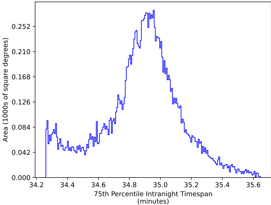
too_elab_r32_d2_gz_v3.4_10yrs WFD: 75th Percentile Intranight Timespan
