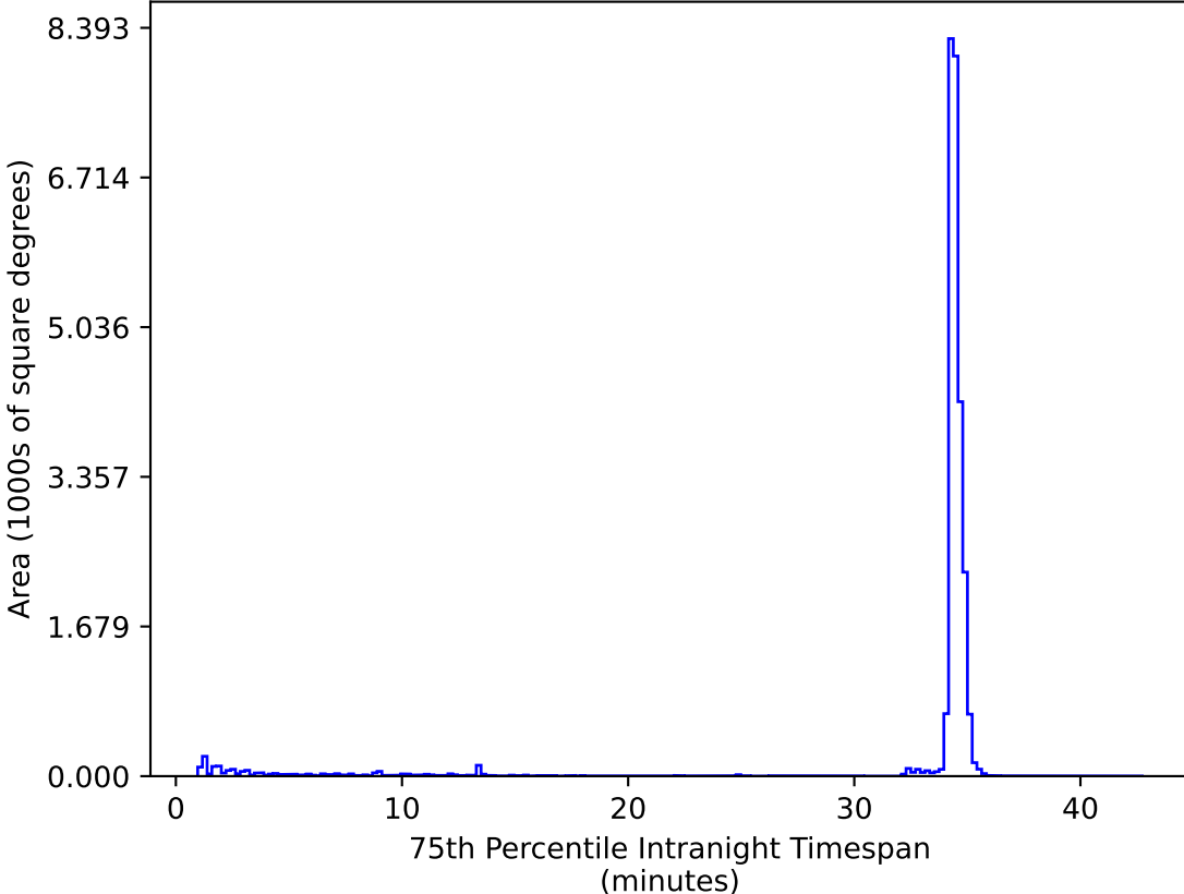
too_elab_r32_d2_gz_v3.4_10yrs All sky zy bands: 75th Percentile Intranight Timespan
