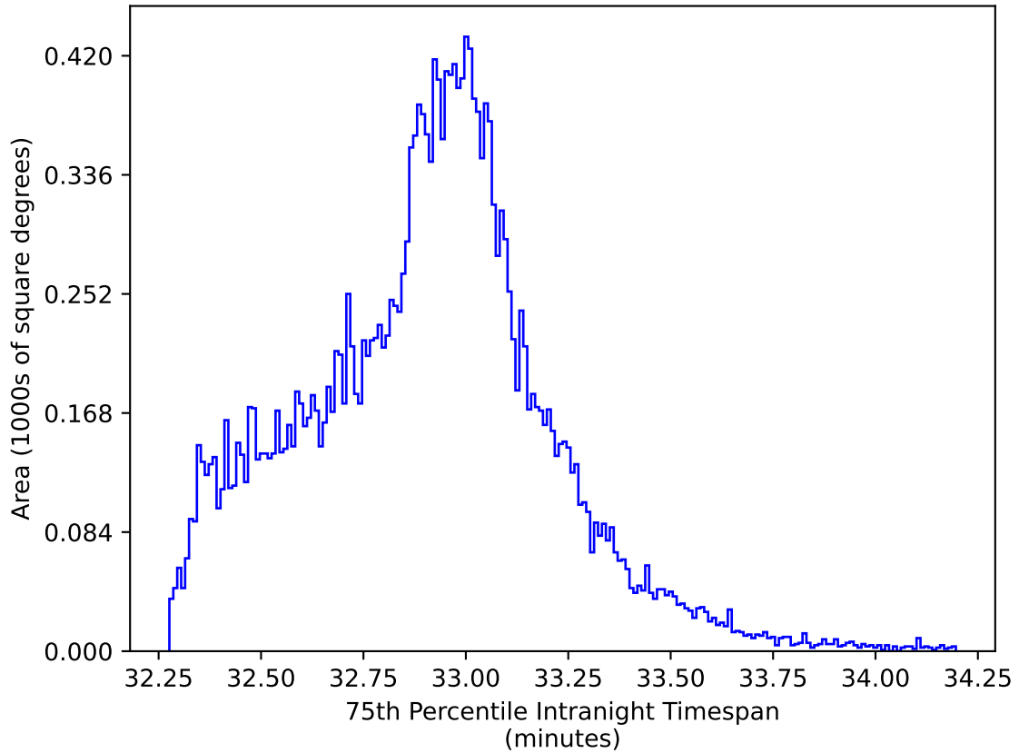
too_elab_r32_d2_gz_v3.4_10yrs All sky y band: 75th Percentile Intranight Timespan
