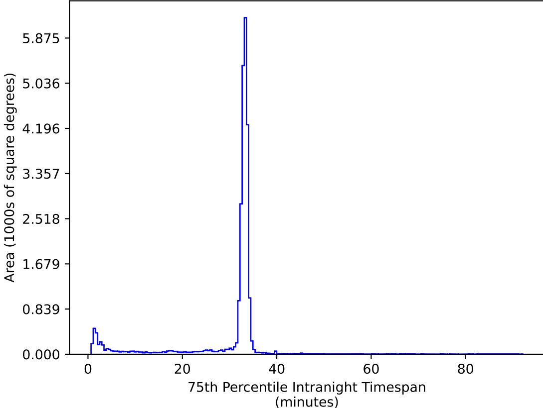
too_elab_r32_d2_gz_v3.4_10yrs All sky ug bands: 75th Percentile Intranight Timespan
