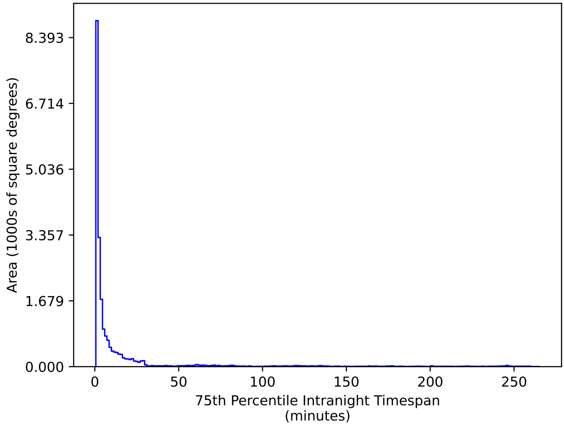
too_elab_r32_d2_gz_v3.4_10yrs All sky u band: 75th Percentile Intranight Timespan
