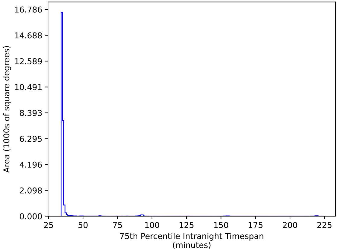
too_elab_r32_d2_gz_v3.4_10yrs All sky ri bands: 75th Percentile Intranight Timespan
