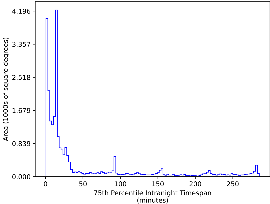
too_elab_r32_d2_gz_v3.4_10yrs All sky r band: 75th Percentile Intranight Timespan
